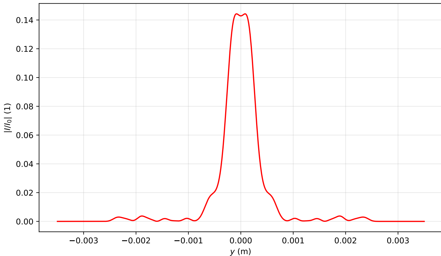
Intensity profile I(x=0, y, z=3.025)/I_0 , P_{in}=6.0P_{cr} , artificial time
